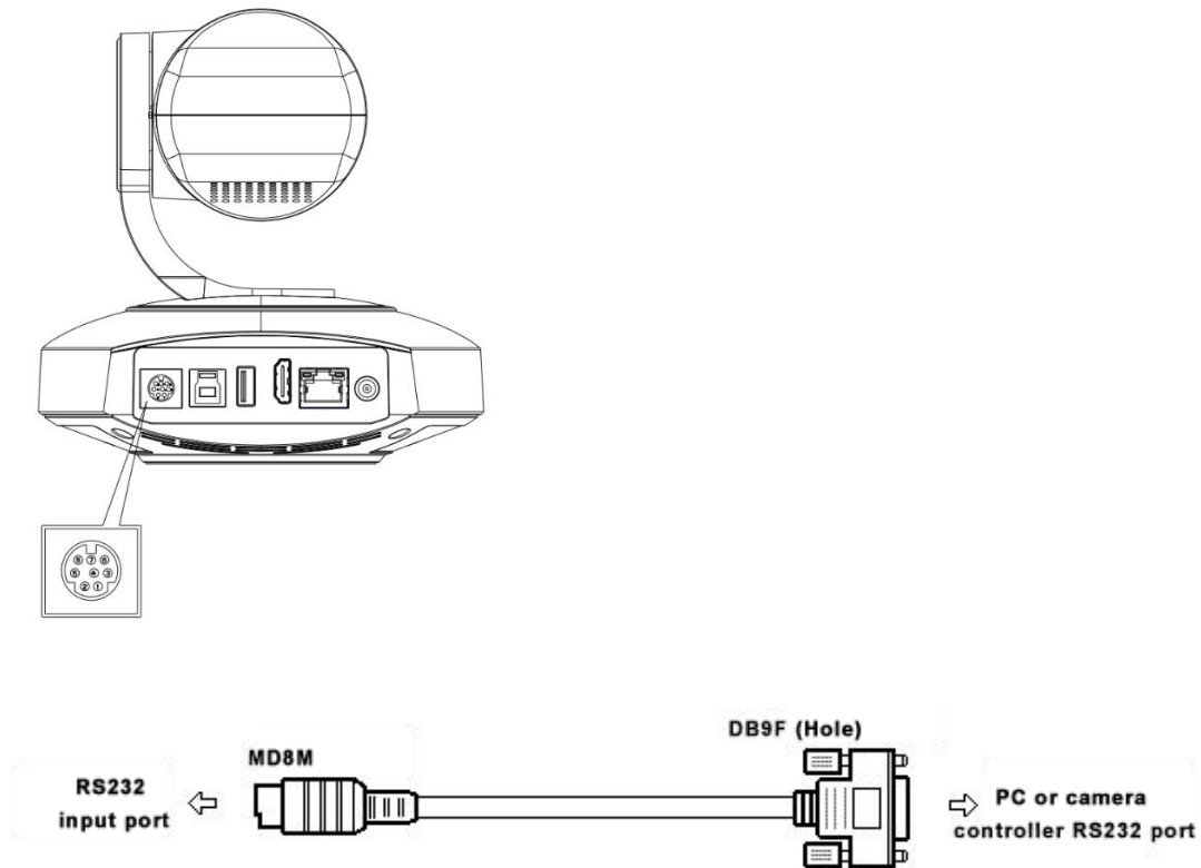
Figure 2-3 RS-232 Diagram
