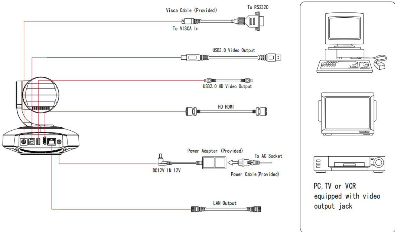
Figure 2-2 Interface Diagram
