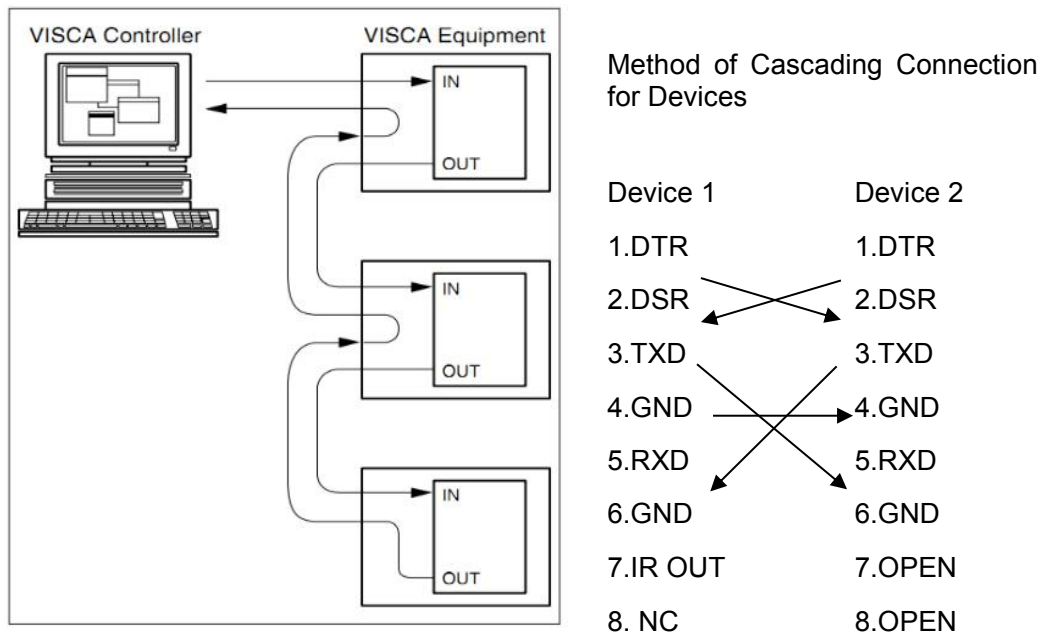
Figure 2-4 VISCA Schematic Diagram of Networking Configuration
