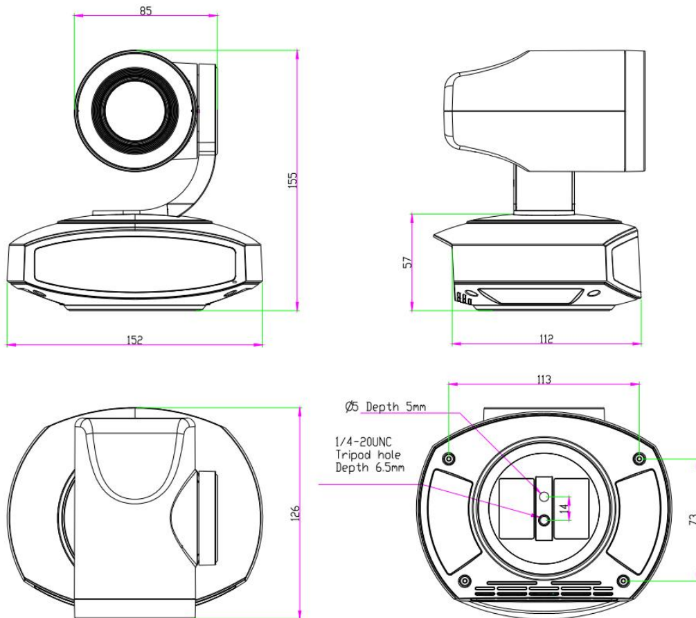
Figure 2-1 Product Dimension
