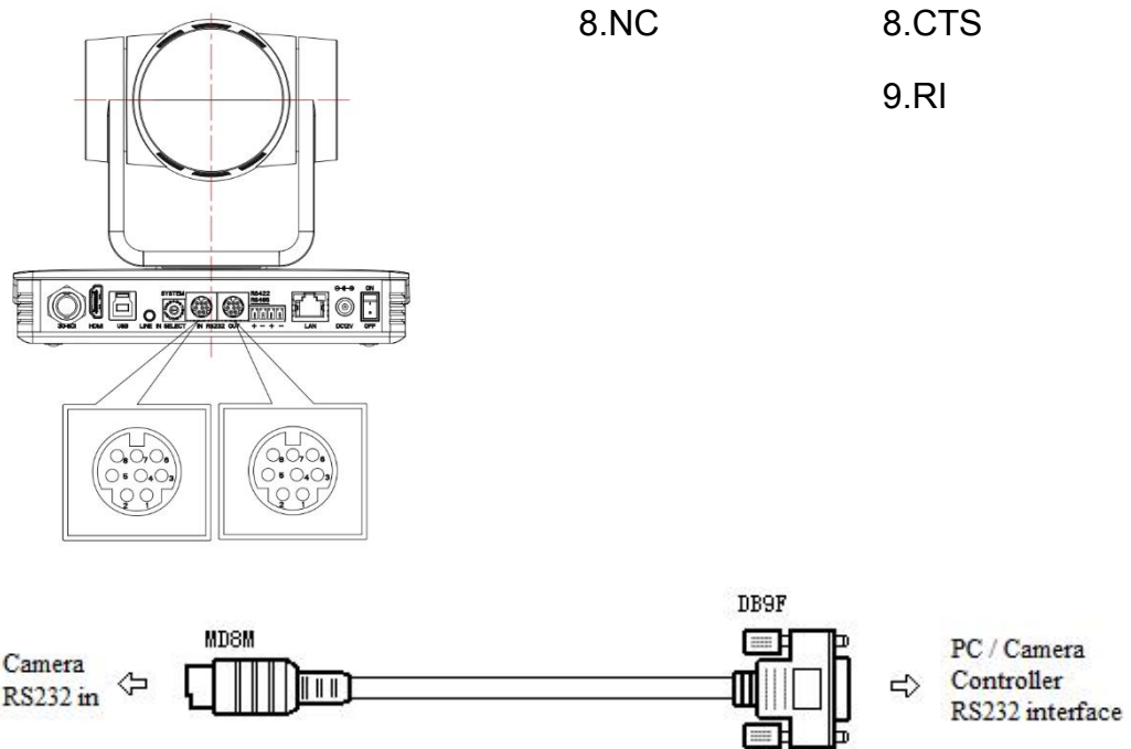
Figure1-6 diagram of RS232 Connection
