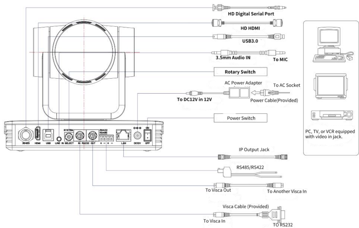
Figure1-5 Back Panel
