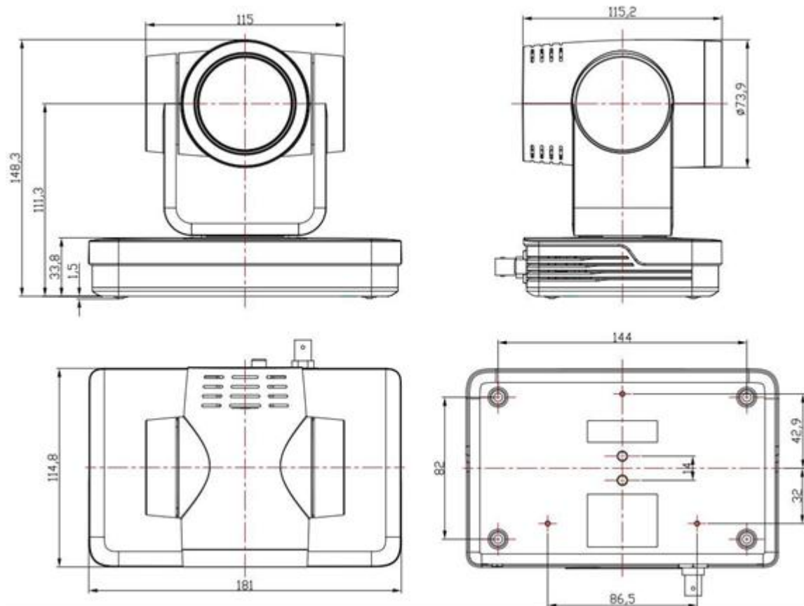
Figure1-4 Product Dimension
