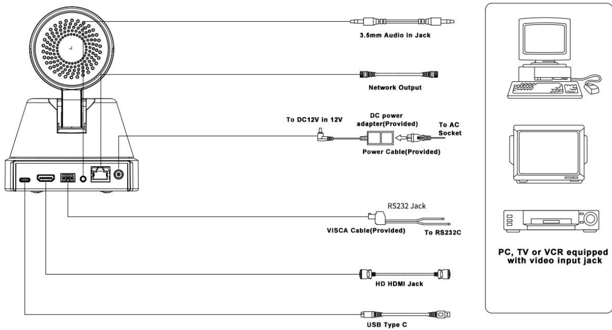
Figure1-5 Interface Diagram
