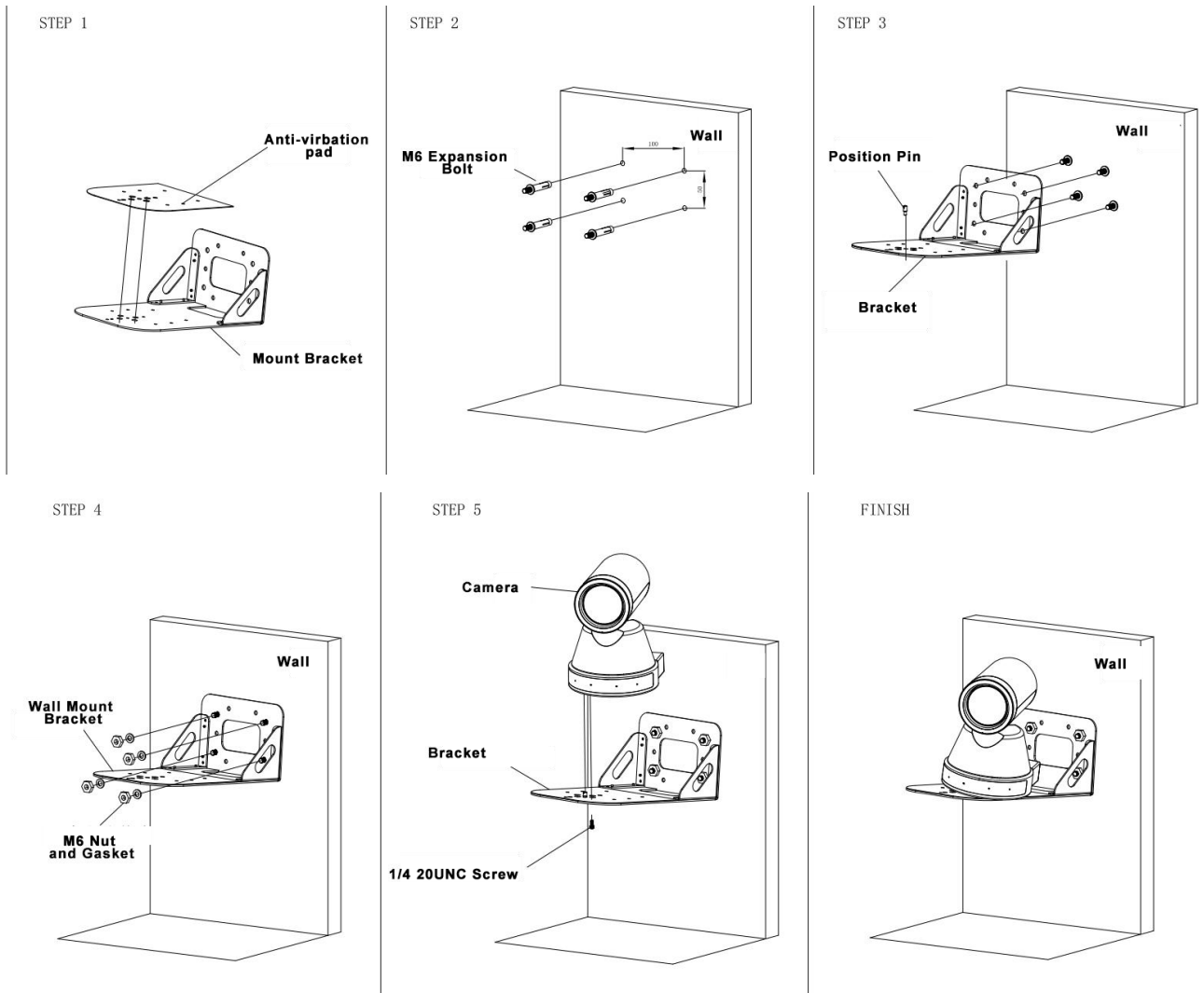
Figure1-2 Steps of Wall Mount
