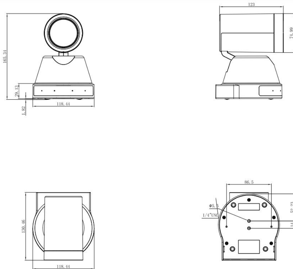
Figure1-4 Product Dimension
